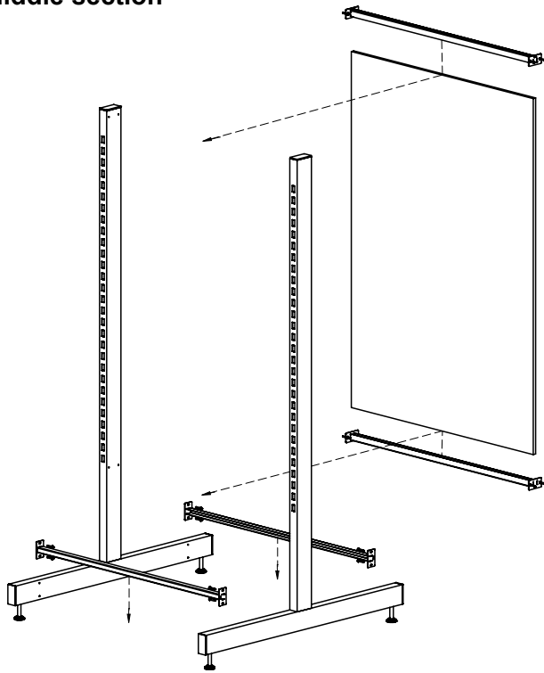
1. Middle section
